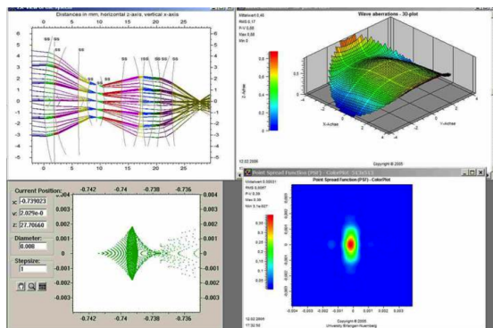
(a) Numerical modeling of an optical objective
