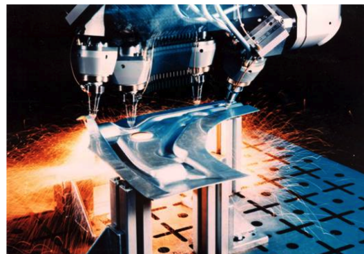
(b) Laser welding in automotive industry
